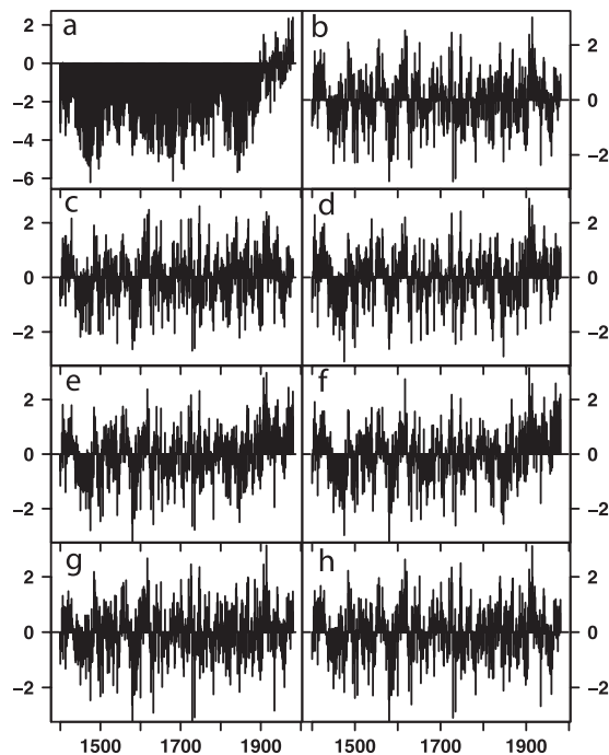
Figure 1. MBH98 North American AD1400 network. (a) MBH98 PC1 centered on 1902–1980 (as in MBH98); (b) same calculation with bristlecone pines removed. (c) Covariance PC1; (d) mean of all 212 series. (e) Correlation PC1; (f) mean of 70 full-length series. (g) Autocorrelation-consistent correlation PC1; (h) correlation PC1 with bristlecone pines censored.
